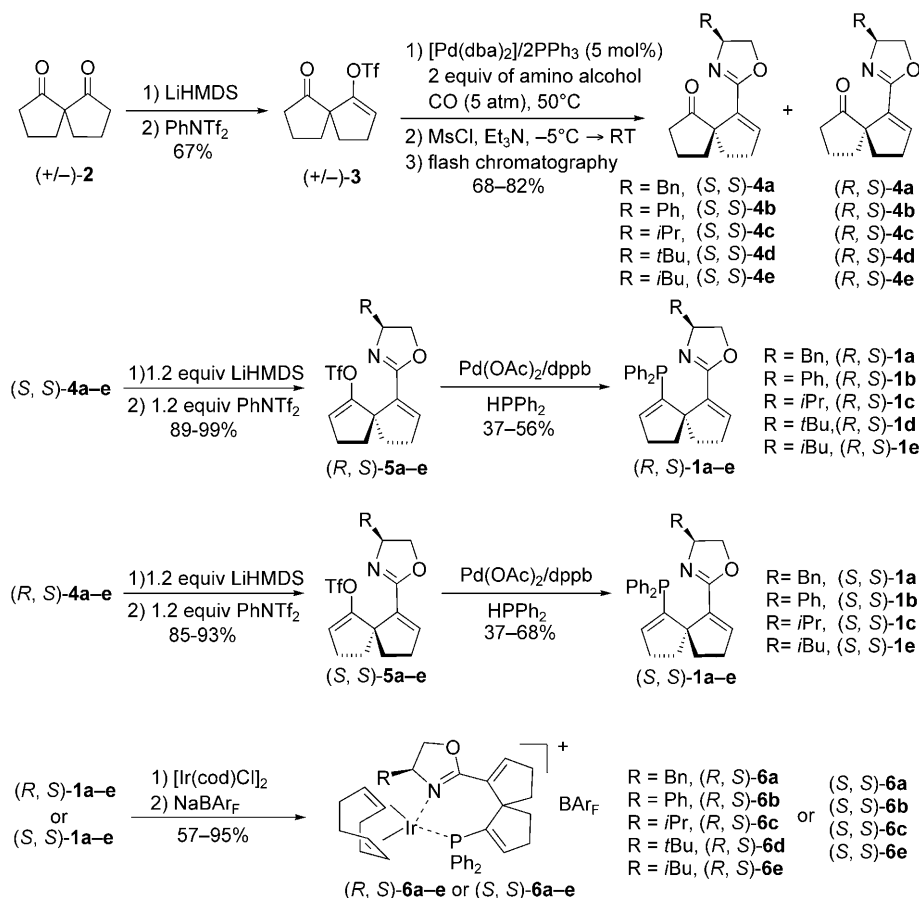
Scheme 2. Synthesis of SpinPHOX ligands ( R,S )- 1 and ( S,S )- 1 and of their Ir I complexes ( R,S )- 6 and ( S,S )- 6 . LiHMDS: lithium hexamethyldisilazane; Tf: trifluoromethanesulfonyl; dba: dibenzylideneacetone; Ms: methanesulfonyl; Bn: benzyl; dppb: 1,1'-bis(diphenylphosphanyl)butane; cod: cycloocta-1,5-diene; NaBAR F : sodium tetrakis(3,5-bis(trifluoromethyl)phenyl)borate.
